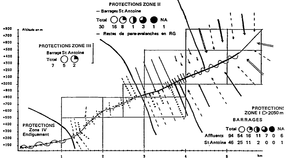
Figure 14.3 : Confrontation "Processus érosifs-protection"
